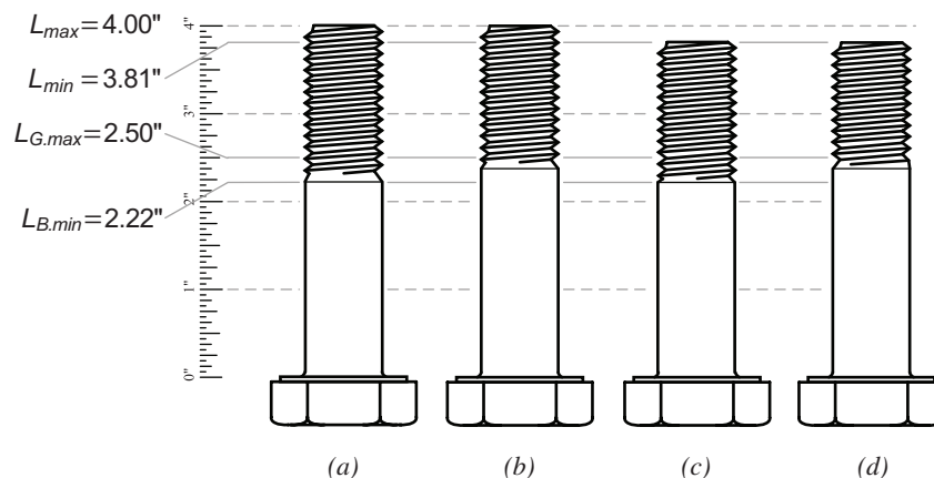
Fig. 7. Different variations of 7/8-in.-9×4-in. high-strength bolts per ASME B18.2.6-19.
