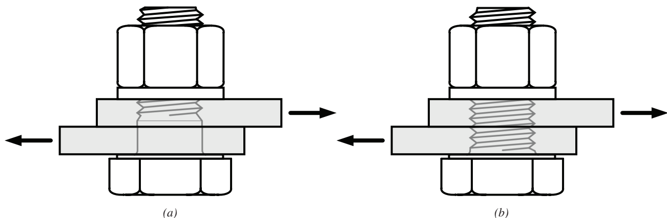
Fig. 6. Illustration of a joint with ⅞-in.-9×2-in. bolts (a) as might be expected by the engineer of record and (b) as provided.
