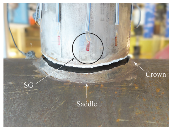
Fig. 3. Weld fracture in a 90° cross-connection.
