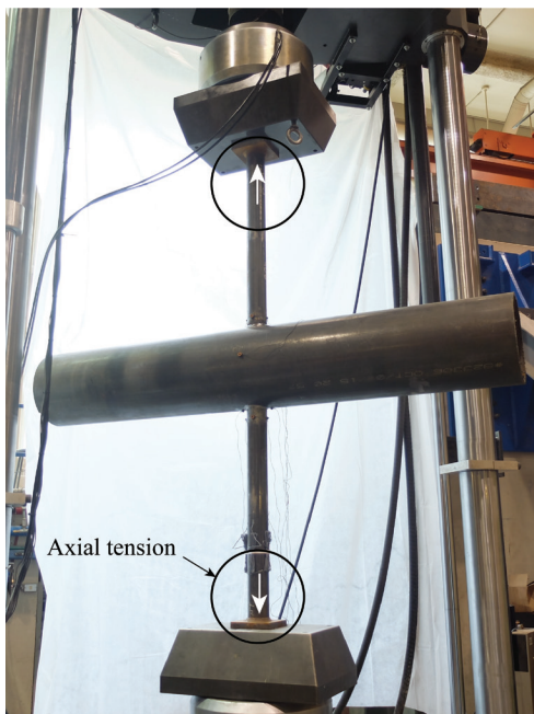
Fig. 2. Testing arrangement for round-to-round HSS cross-connections.
