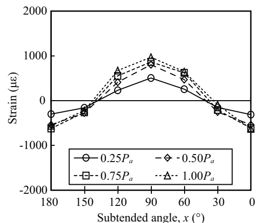
Fig. 4. Strain distribution around the weld, for a HSS5.00x0.500 branch to HSS10.75x0.500 chord.
