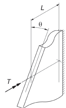
Fig. 3. Torsional deformation of a connection element.
