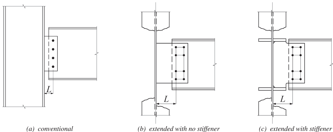
Fig. 10. Single-plate connections.
