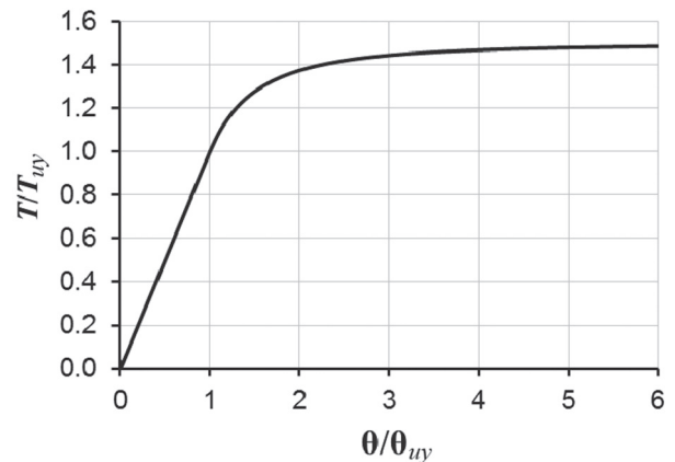
Fig. 1. Normalized torsion versus normalized angle of twist (Dowswell, 2015).
