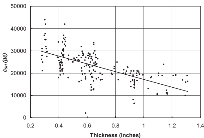
Fig. 7: Strain at onset of strain hardening versus coupon thickness.
