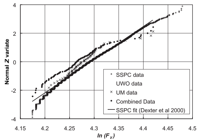
Fig. 6: CDF for ultimate tensile strength data.
