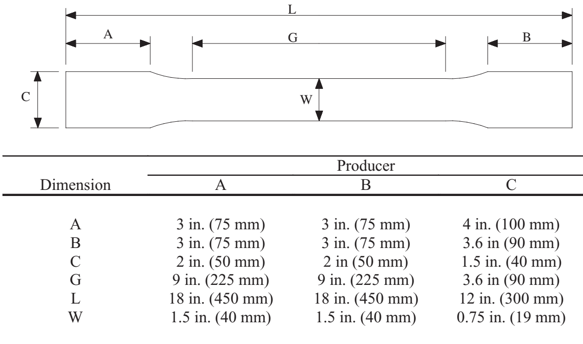
Fig. 2: Coupon geometry.
