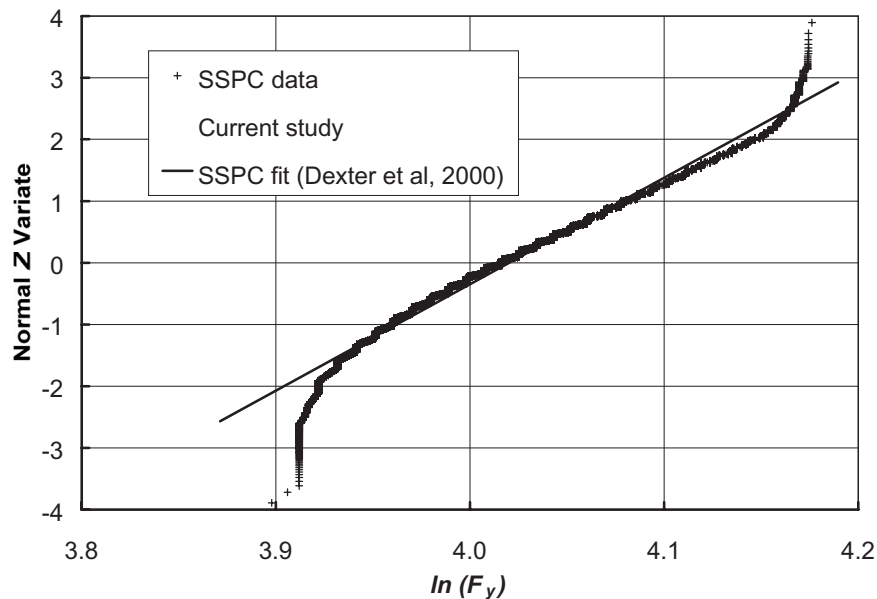
Fig. 4: CDF for yield strength data.
