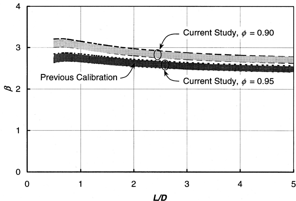
Fig. 9: Variation of \phi with L/D , braced compact beams.
