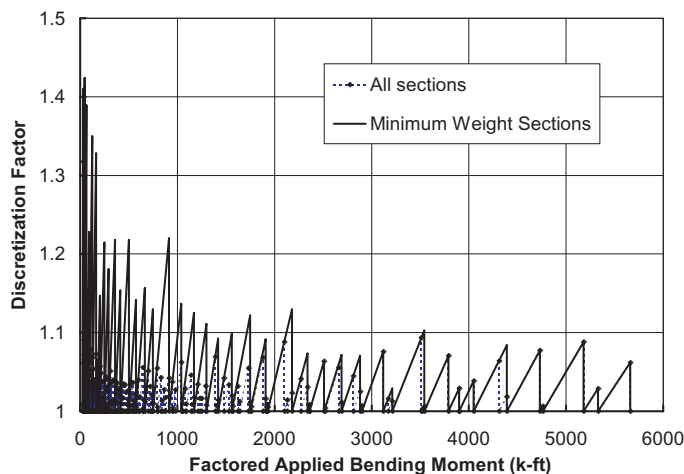
Fig. 8: Discretization factor for braced compact beams.
