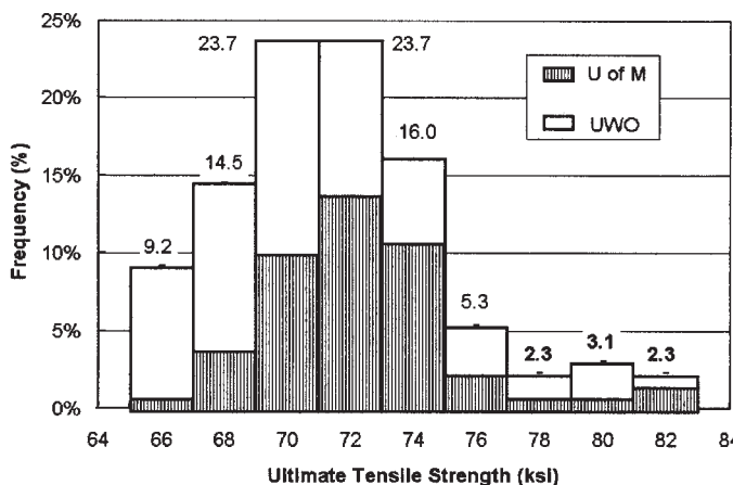
Fig. 5: Histogram of ultimate tensile strength data.
