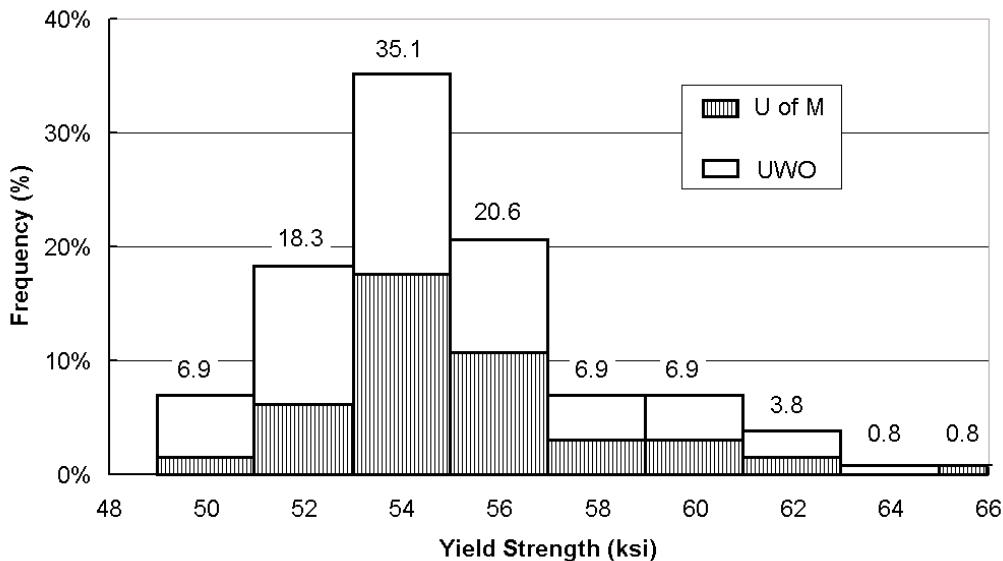
Fig. 3: Histogram of yield strength data.
