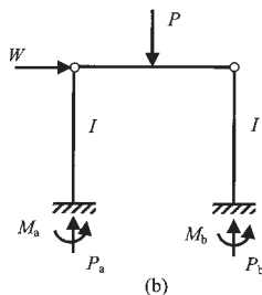
Fig. 6. Symmetric Portal Frame
