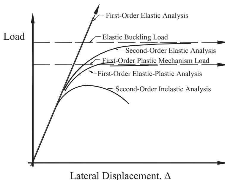
Fig. 1. Load-displacement history.
