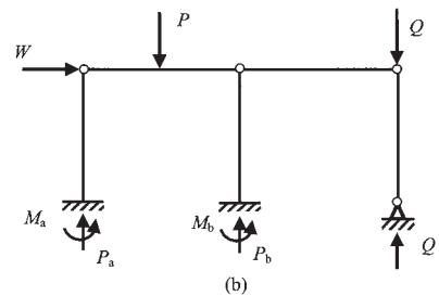
Fig. 7. Symmetric Frame with Leaning Column
