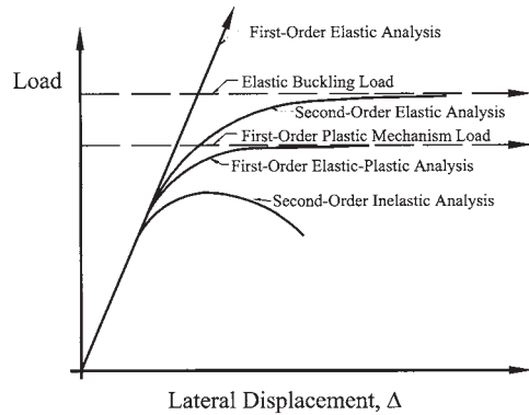
Fig. 1. Load-Displacement History
