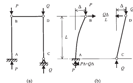
Fig. 9. Equilibrium Forces for Yura Derivation
