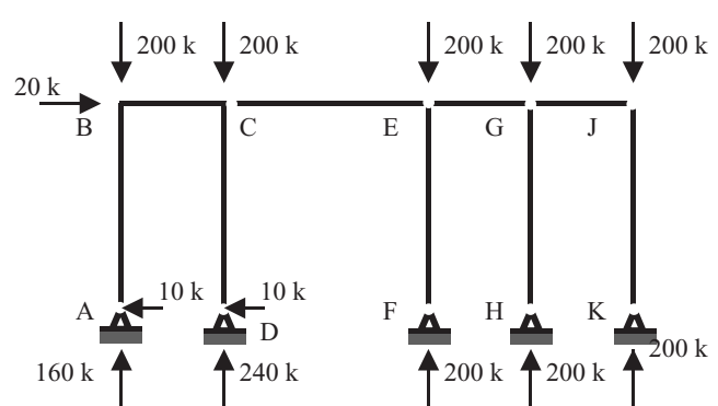
Fig. 11. Example 2 frame with gravity and lateral load and reactions from a first order analysis.
