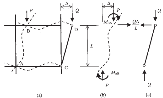
Fig. 8. Restraining and Leaning Columns
